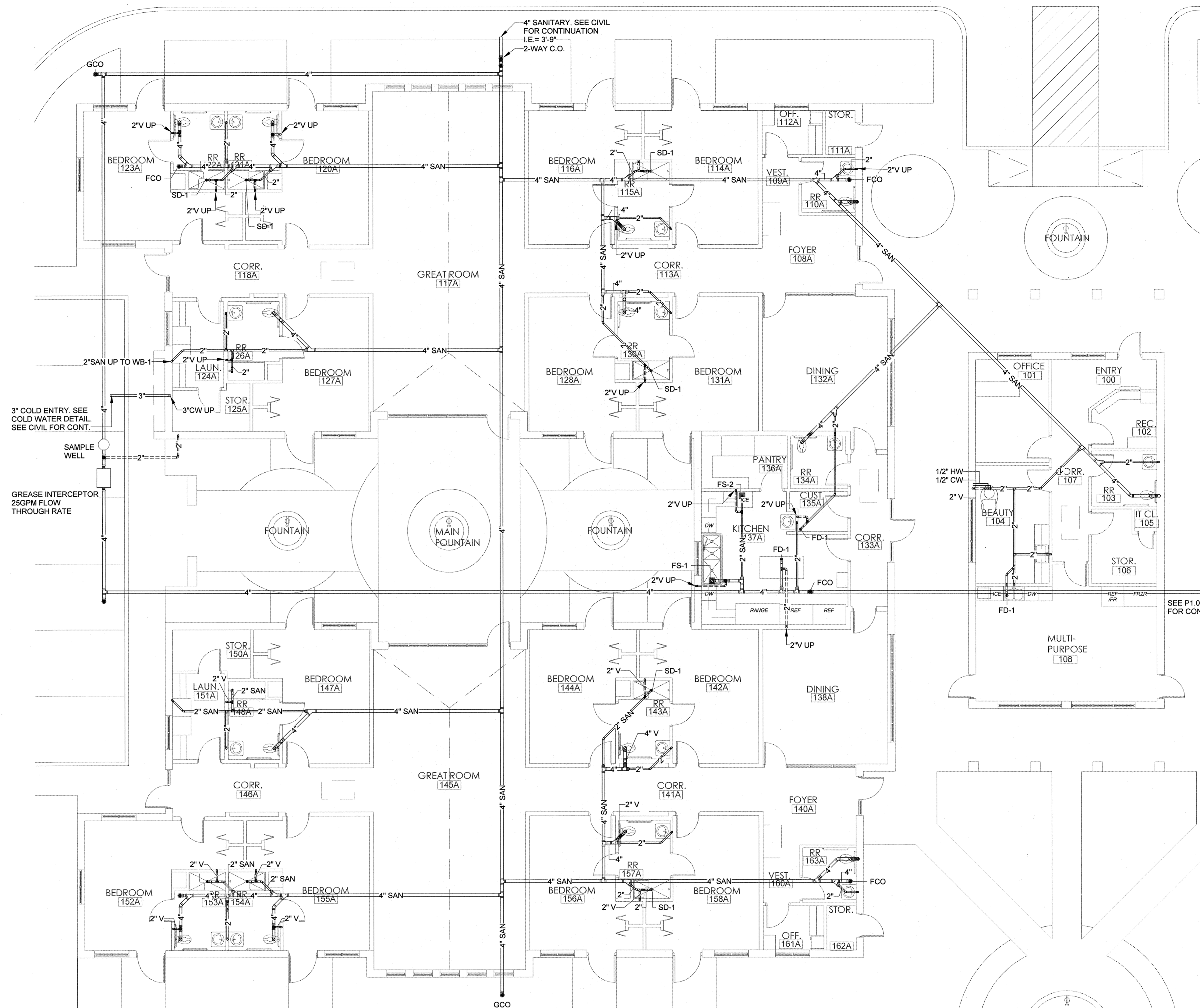
1 PLUMBING PLAN - AREA A - BELOW FLOOR 1/8" = 1'-0"
